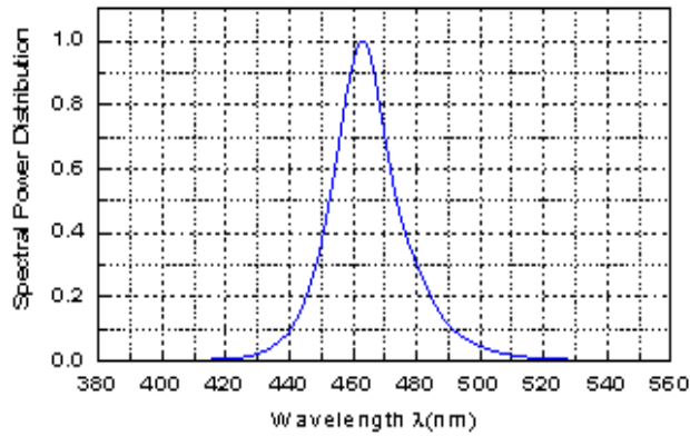
Figure3. Spectral Power Distribution VS. Wavelength
