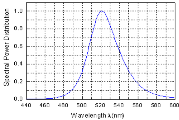
Figure3. Spectral Power Distribution VS. Wavelength
