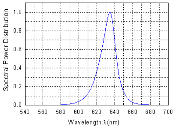
Figure3. Spectral Power Distribution VS. Wavelength
