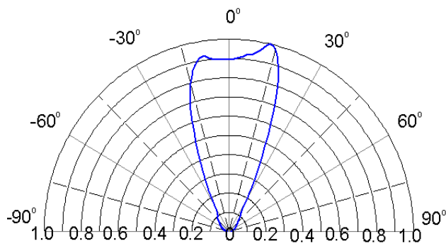
Figure4. Relative Luminosity VS. Radiation Angle
