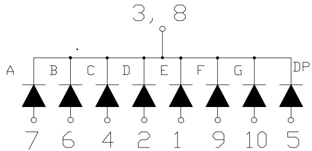
CSOS-S39127 is Common Cathode
