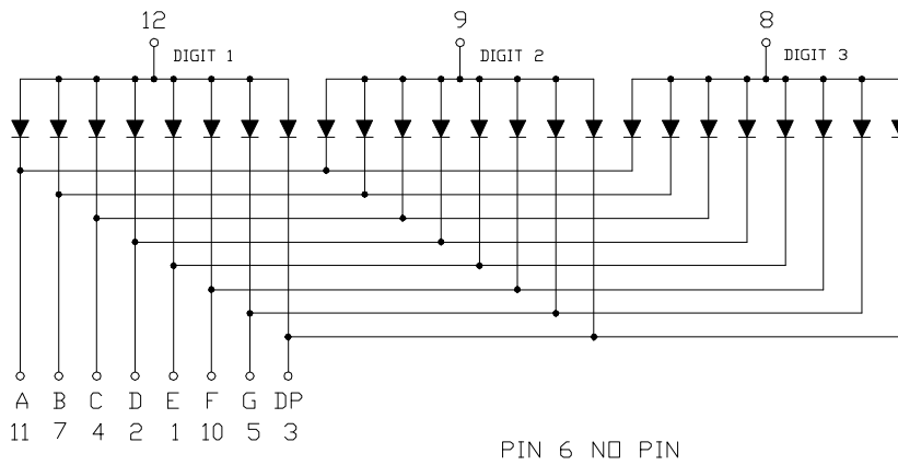
CSDT-36300 is Common Anode
