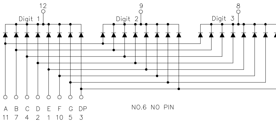
CSDT-36300 is Common Anode
