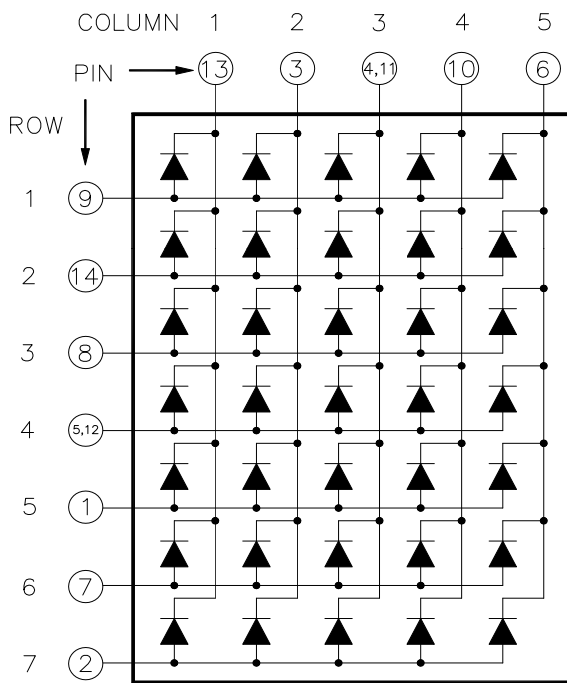
CSOM-57104 is Common Column Cathode
