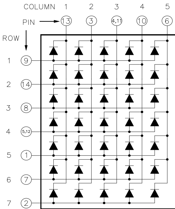
CSOM-57200 is Common Column Cathode
