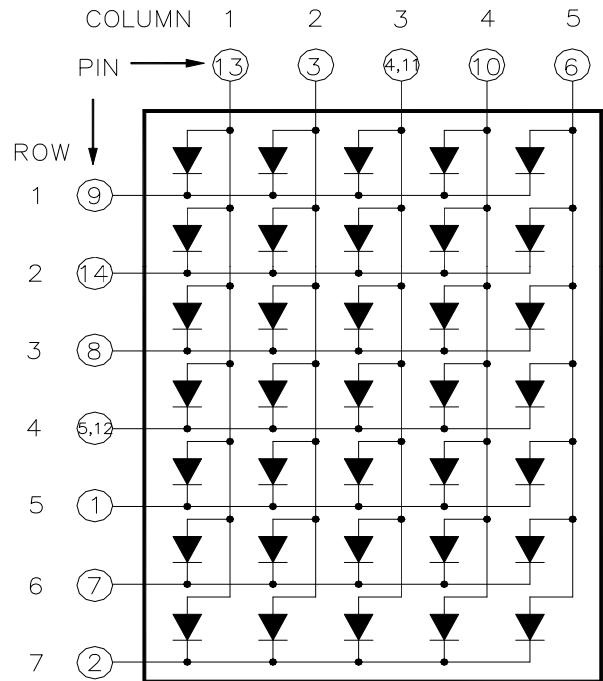
CSOM-57201 is Common Column Anode
