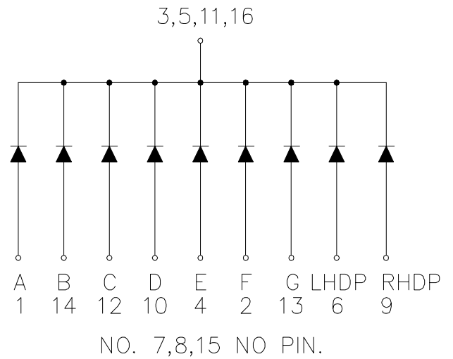
CSOS-56101 is Common Cathode
