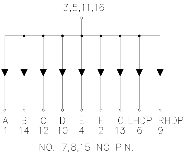
CSOS-80100 is Common Anode
