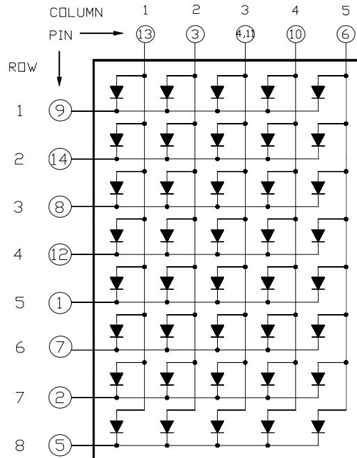
CSDM-58201 is Common Column Anode
