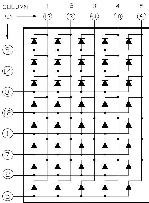
CSOM-58200 is Common Column Cathode
