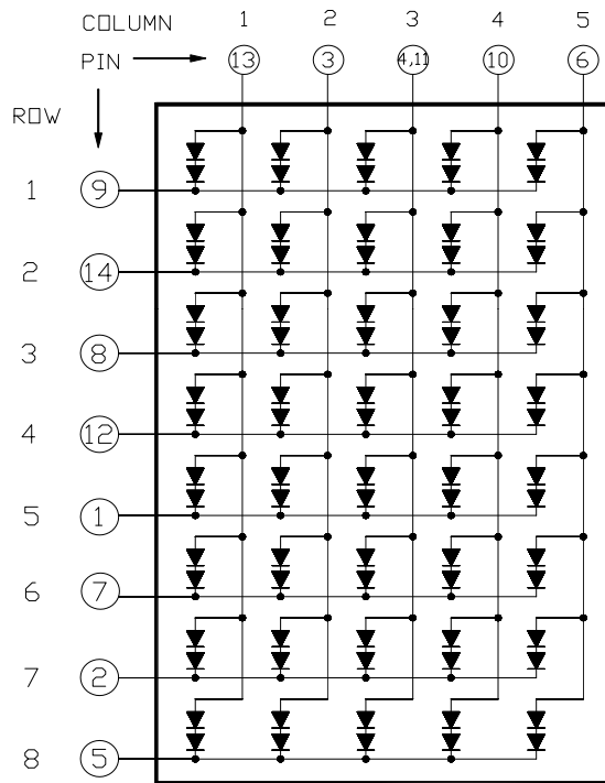
CSDM-58401 is Common Column Anode
