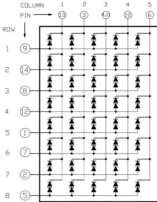
CSOM-58400 is Common Column Cathode
