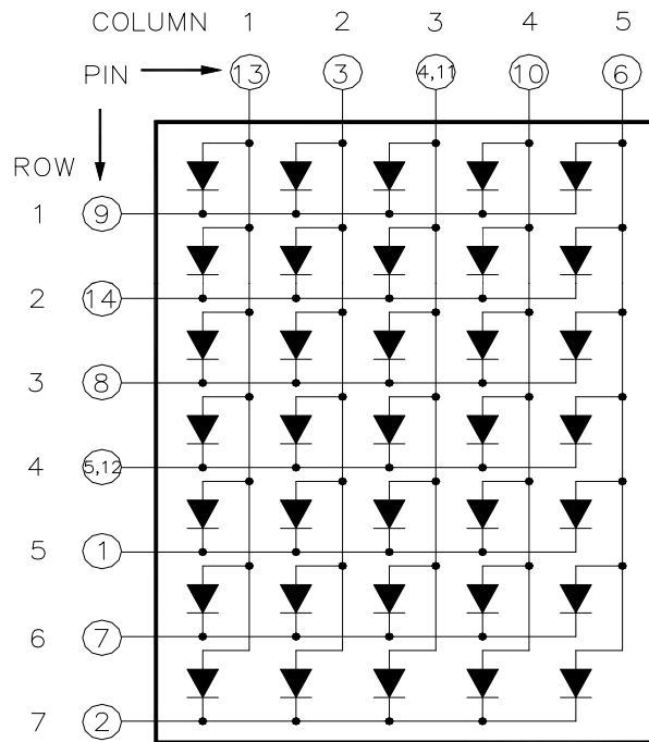
CSOM-57105 is Common Column Anode
