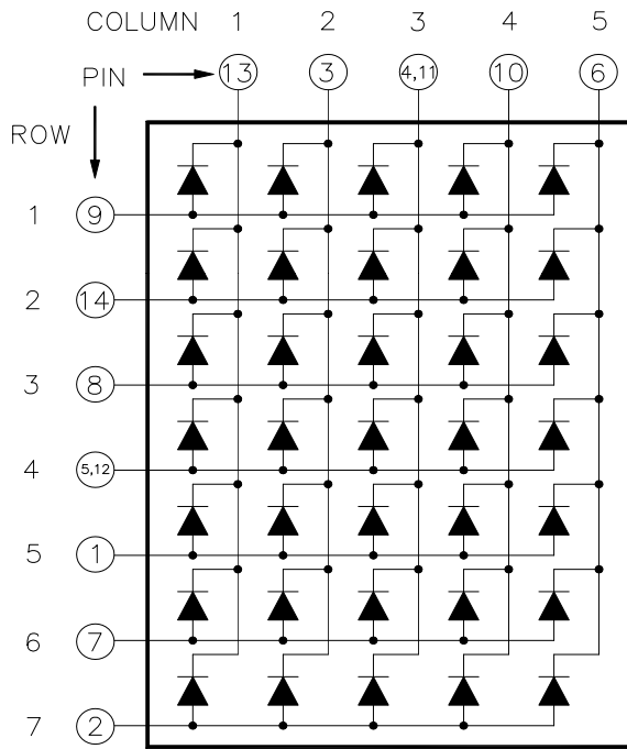
CSOM-57104 is Common Column Cathode
