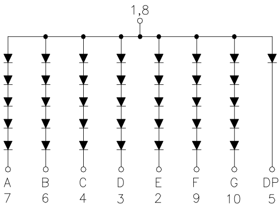
CSOS-4A100 is Common Anode
