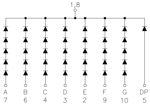
CSOS-4A101 is Common Cathode
