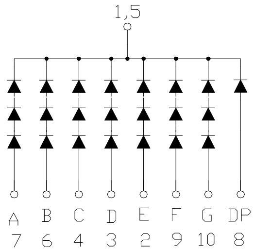
CSOS-1J101 is Common Cathode
