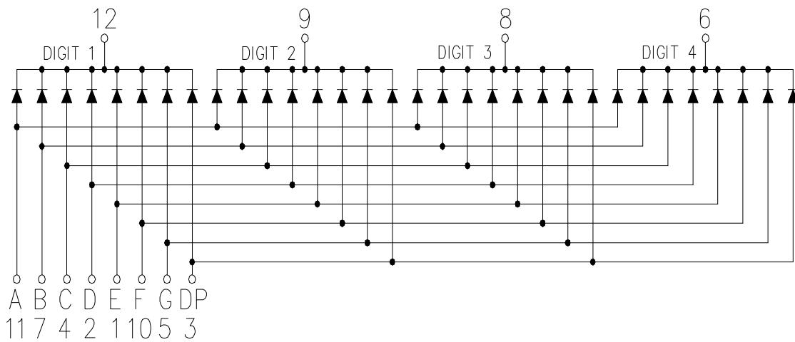
CSOQ-56401 is Common Cathode
