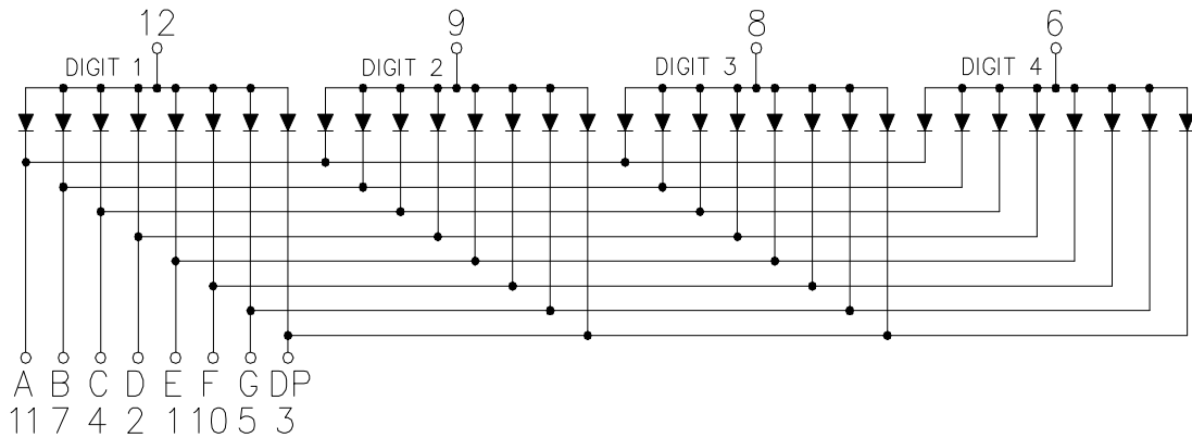
CSOQ-56400 is Common Anode
