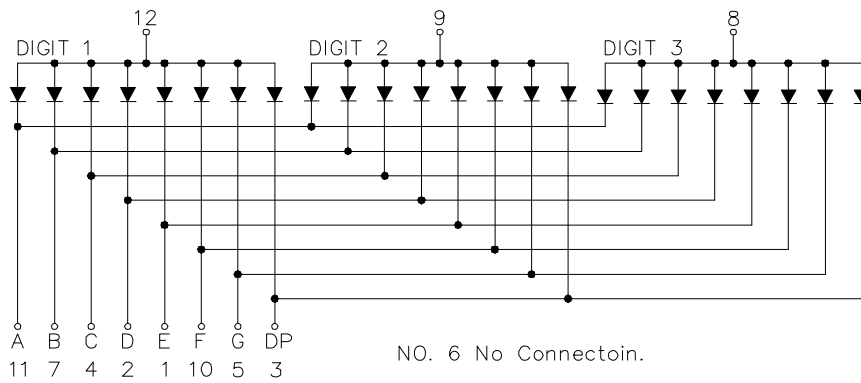
CSDT-80300 is Common Anode
