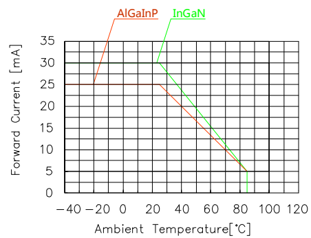
Fig 6. Forward current vs. Temperature
