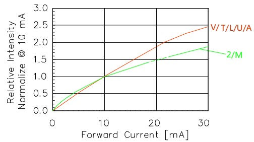
Fig 2. Relative Intensity vs. Forward Current
