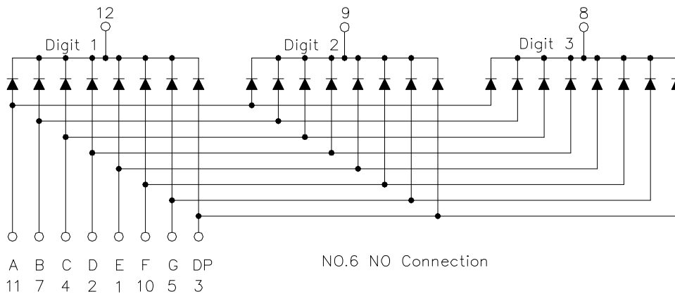
CSDT-80301 is Common Cathode
