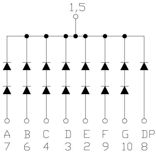
CSDS-1F101 is Common Cathode
