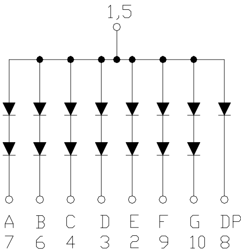
CSDS-1F100 is Common Anode
