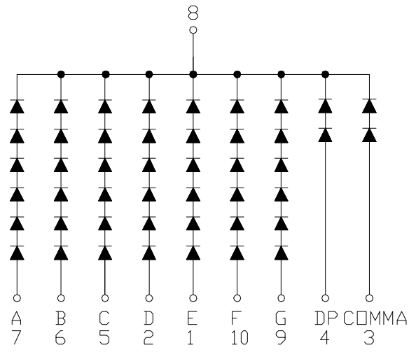
CSDS-3A101 is Common Cathode
