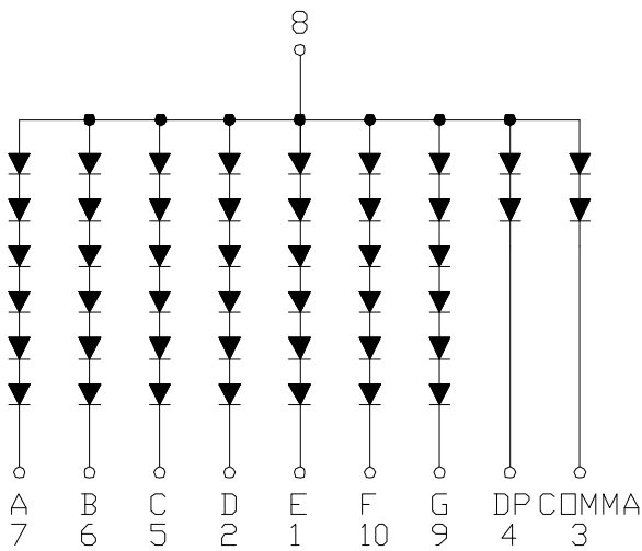
CSDS-3A100 is Common Anode
