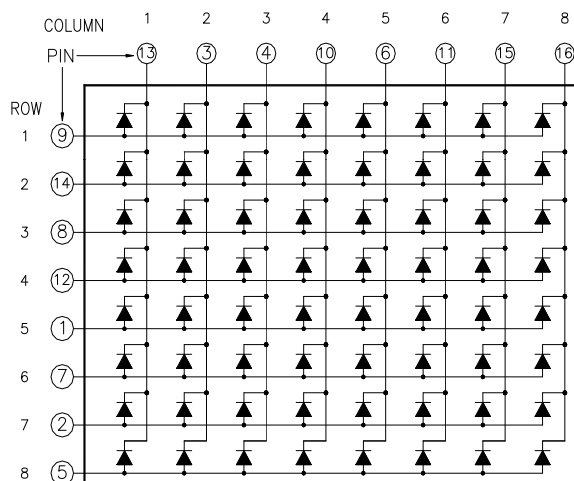
CSDM-88106 is Common Column Cathode
