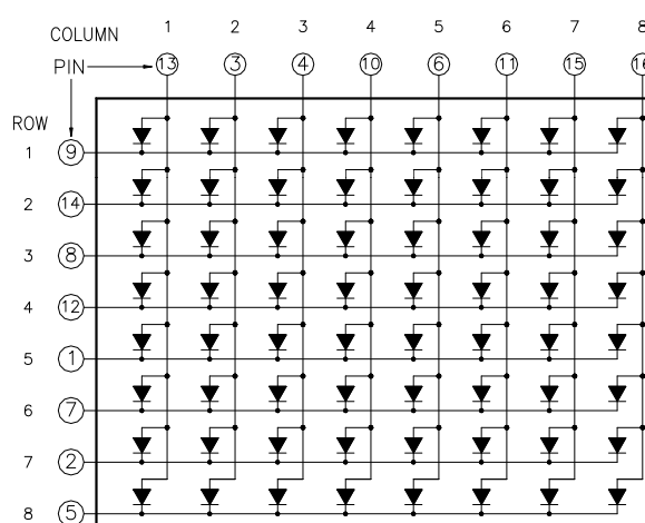
CSDM-88107 is Common Column Anode
