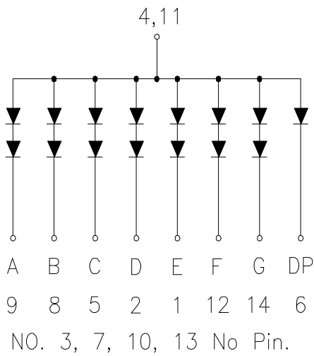
CSOS-1A102 is Common Anode
