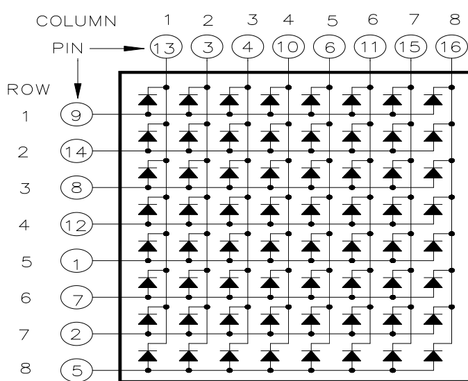
CSDM-88002 is Common Column Cathode
