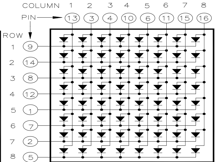
CSDM-88003 is Common Column Anode
