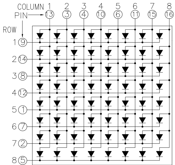
CSOM-88101 is Common Column Anode
