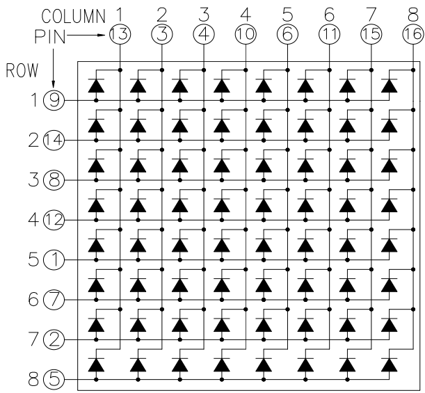
CSOM-88100 is Common Column Cathode
