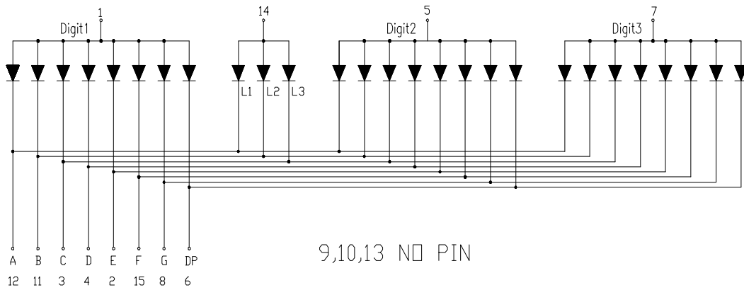
CSDT-39300 is Common Anode
