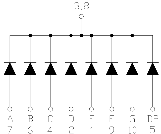
CSOS-52101 is Common Cathode
