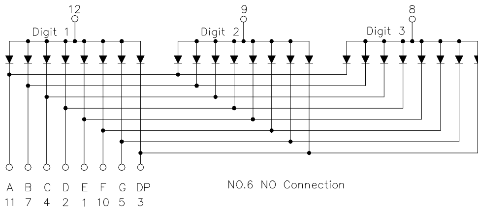
CSDT-56300 is Common Anode
