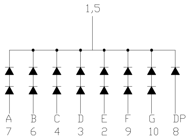
CSOS-1C101 is Common Cathode
