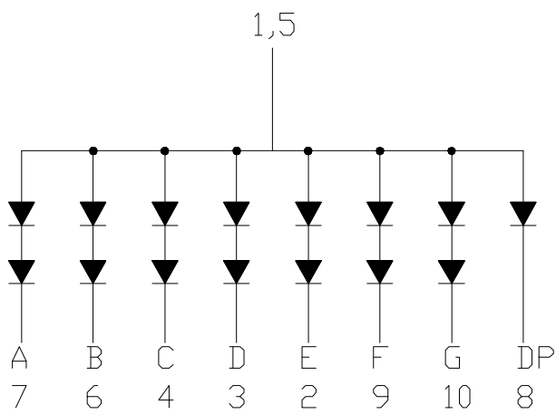
CSOS-1C100 is Common Anode
