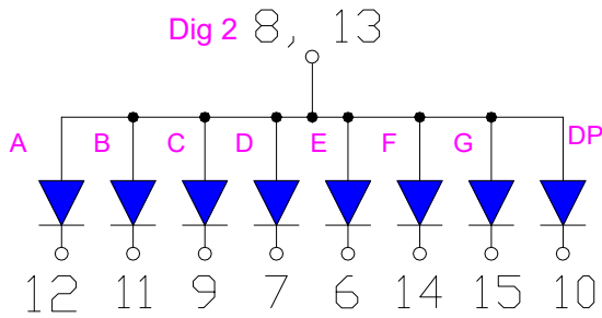
CSOD-S40224 is Common Anode
