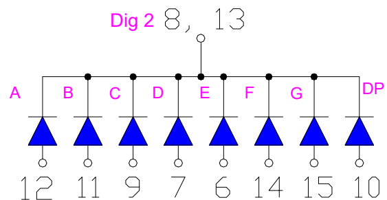
CSOD-S40225 is Common Cathode
