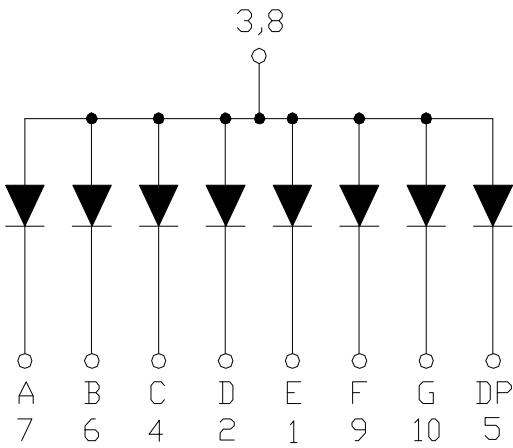
CSDS-52100 is Common Anode
