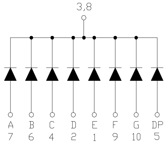
CSDS-52101 is Common Cathode
