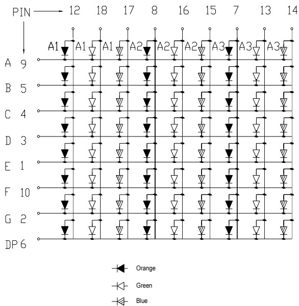
CSDT-S56326 is Common Anode
