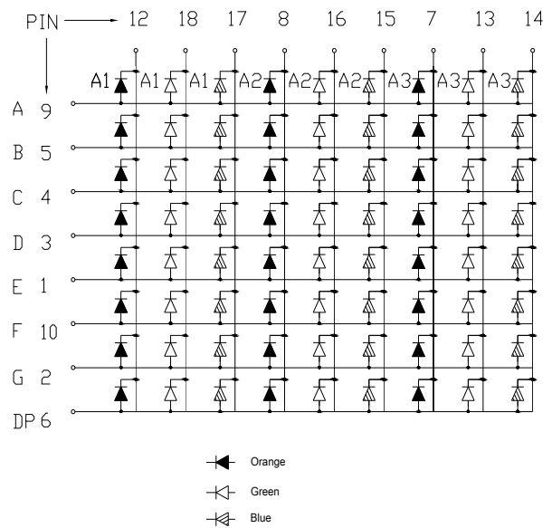
CSDT-S56327 is Common Cathode
