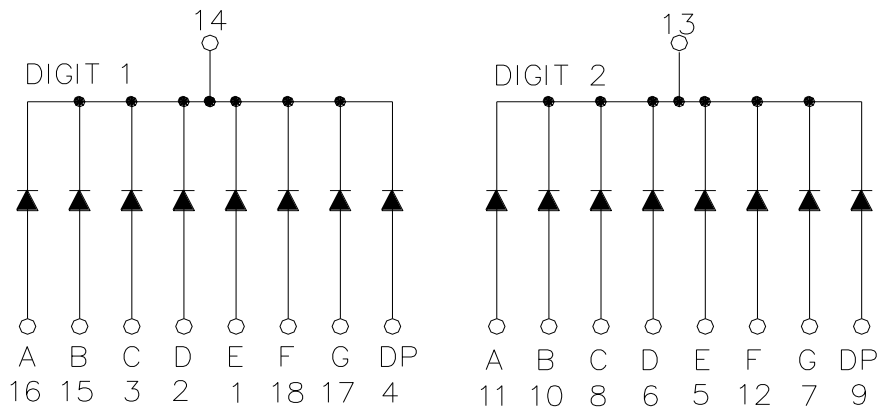
CSOD-56203 is Common Cathode
