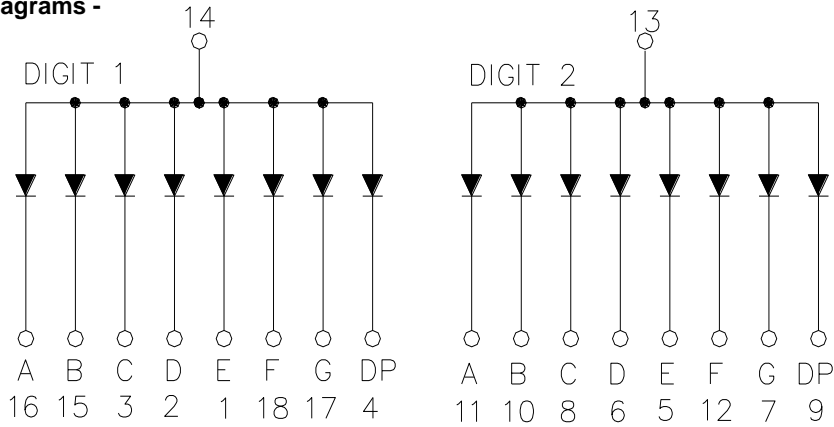
CSOD-56202 is Common Anode
