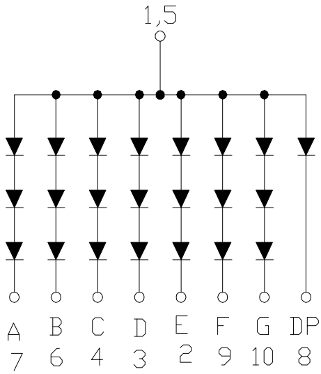
CSOS-1J100 is Common Anode
