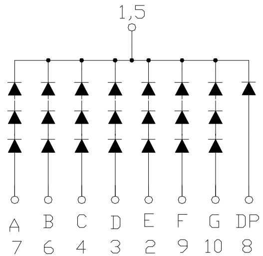
CSOS-1J101 is Common Cathode
