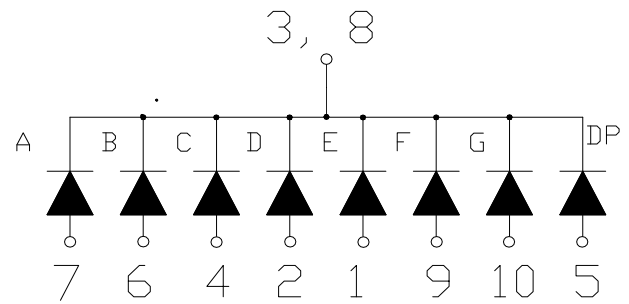
CSOS-S56125 is Common Cathode
