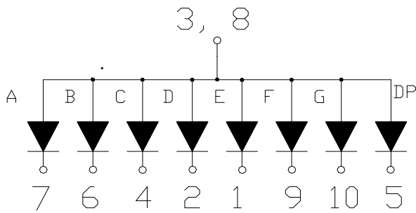
CSOS-S56124 is Common Anode
