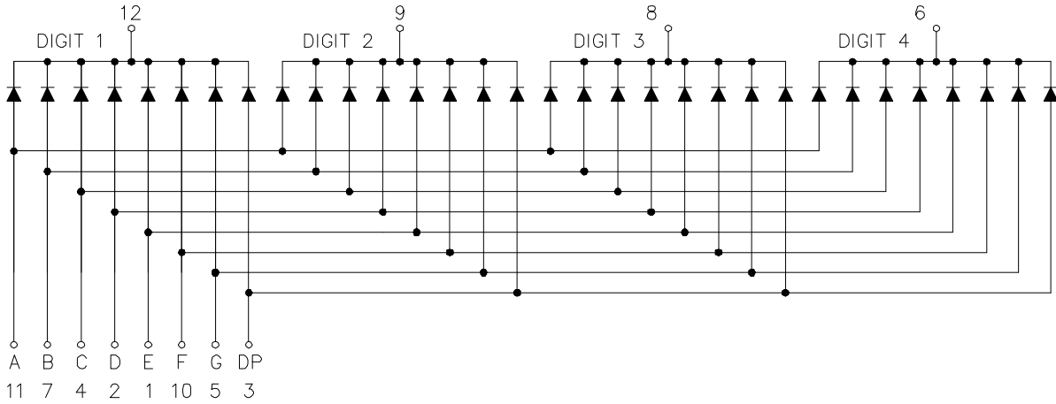
CSOQ-36407 is Common Cathode
