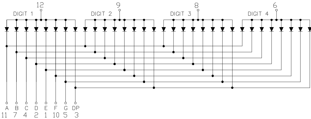
CSOQ-36406 is Common Anode
