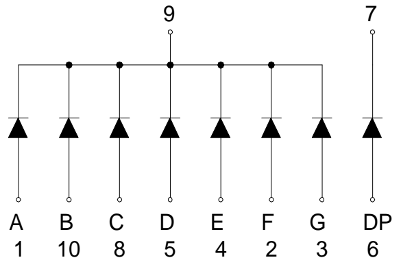
CSOS-31101 is Common Cathode
