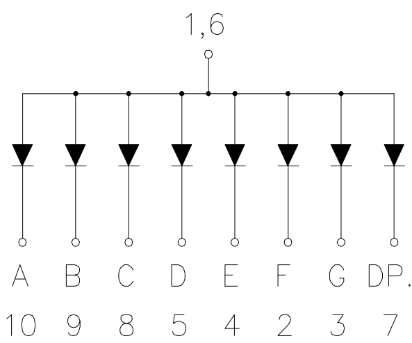
CSDS-40100 is Common Anode
