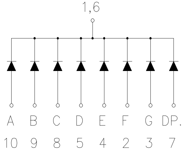
CSDS-40101 is Common Cathode
