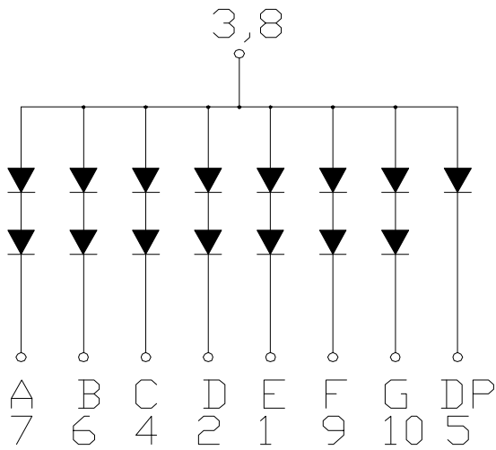
CSDS-1A100 is Common Anode
