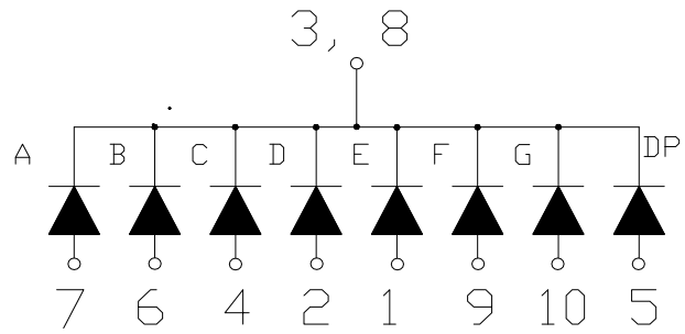
CSOS-S20123 is Common Cathode
