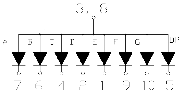
CSOS-S20122 is Common Anode
