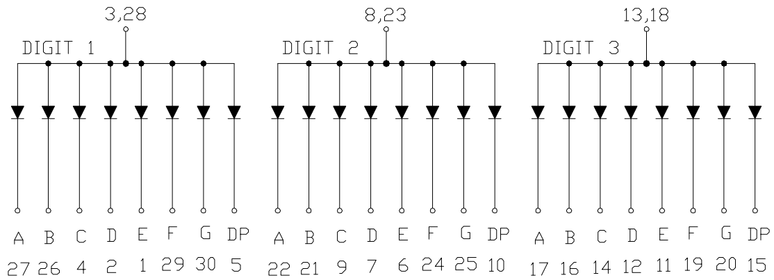
CSDT-52300 is Common Anode
