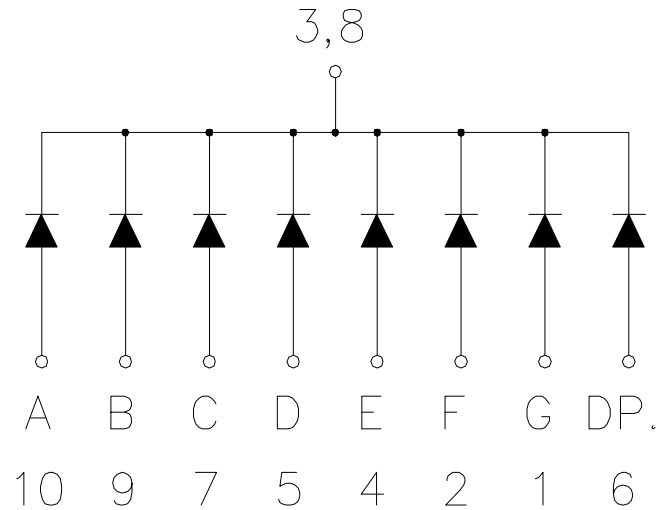
CSOS-39101 is Common Cathode
