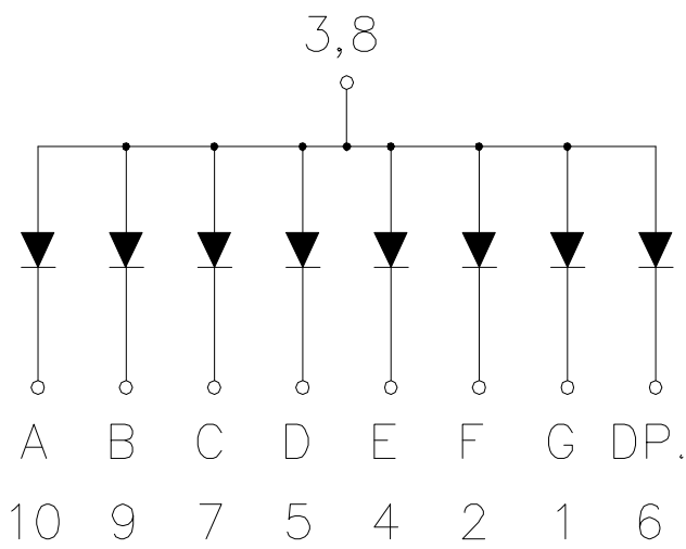
CSOS-39100 is Common Anode
