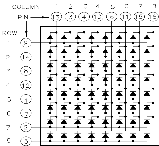
CSDM-88114 is Common Column Cathode
