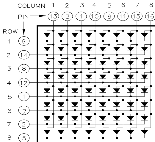
CSDM-88115 is Common Column Anode
