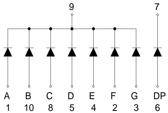
CSDS-31101 is Common Cathode
