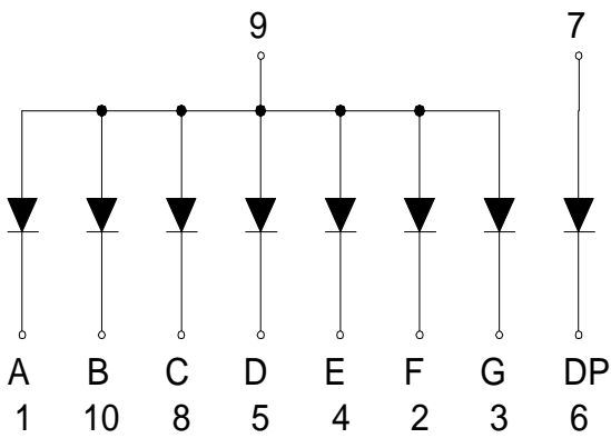
CSDS-31100 is Common Anode
