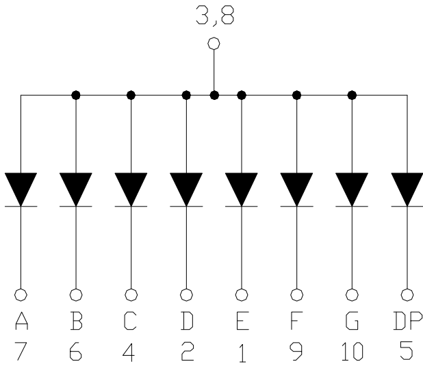
CSOS-52100 is Common Anode
