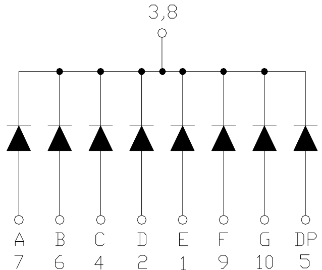
CSOS-52101 is Common Cathode
