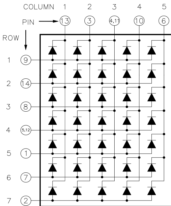
CSOM-57100 is Common Column Cathode
