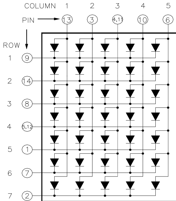
CSOM-57101 is Common Column Anode
