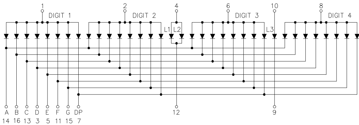
CSOQ-39400 is Common Anode
