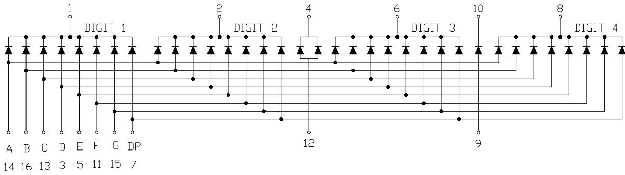
CSOQ-39401 is Common Cathode
