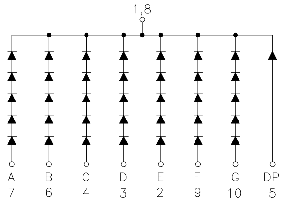
CSOS-4A101 is Common Cathode
