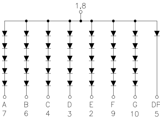
CSOS-4A100 is Common Anode
