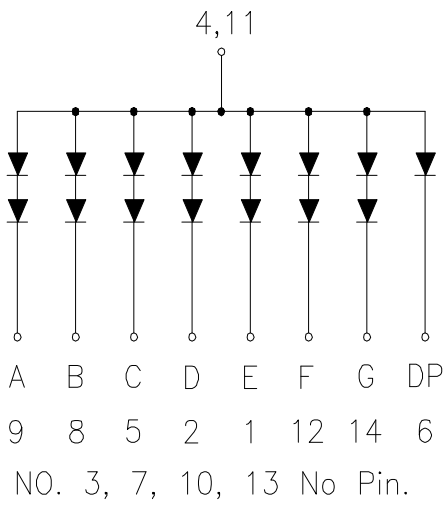
CSDS-1A102 is Common Anode
