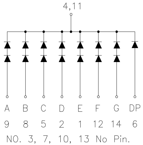
CSDS-1A103 is Common Cathode
