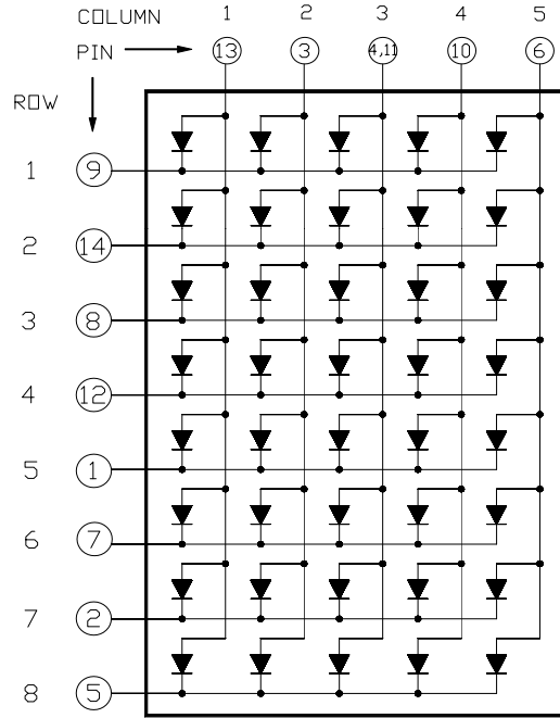
CSOM-58201 is Common Column Anode
