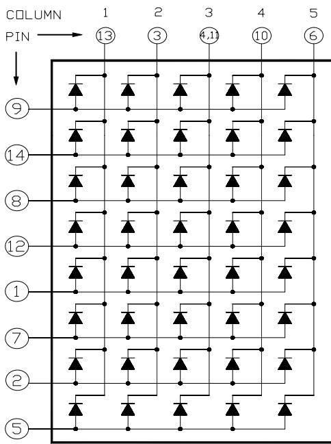
CSOM-58200 is Common Column Cathode
