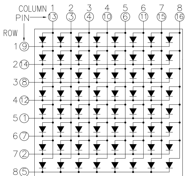
CSOM-88007 is Common Column Anode
