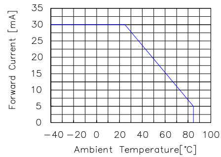
Fig 6. Forward current vs. Temperature
